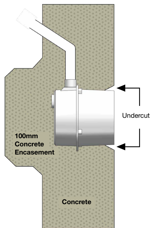
Diagram 1 – After Concreting
