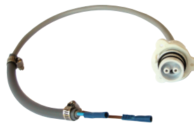
8. Extension Cable Joining Kit. 60cm long to extend the original cable. Available in 1mm 2 (P/N LED114), 1.5mm 2 (P/N LED115) and 4mm 2 (P/N LED120).
