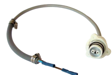
11. Extension Cable Joining Kit. 60cm long to extend the original cable. Available in 1mm 2 (P/N LED114), 1.5mm 2 (P/N LED115) and 4mm 2 (P/N LED120).
